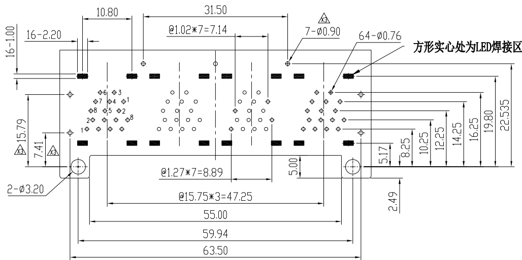
RECOMMENDED PCB LAYOUT (VIEWED FROM COMPONENT SIDE) TOLERANCE \pm 0.05 THICKNESS=1.6MM
